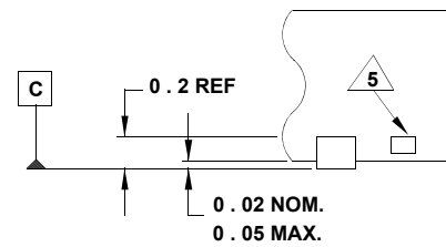
DETAIL "X"
