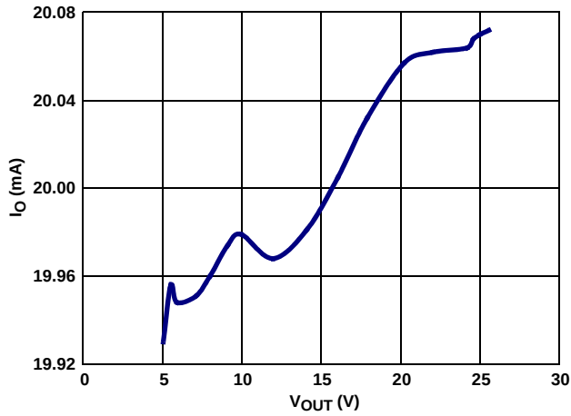
FIGURE 3. LOAD REGULATION ( V_{IN} = 4V )
