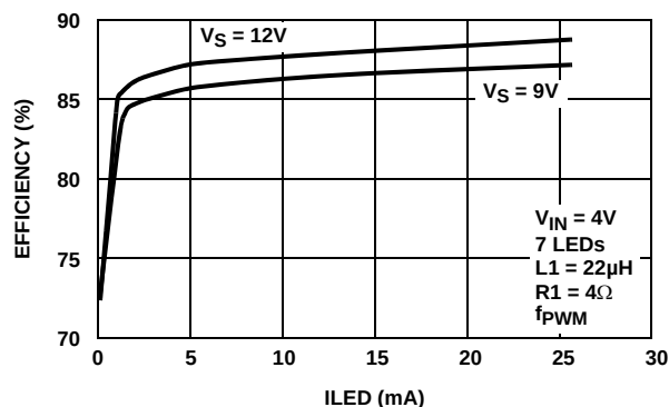
FIGURE 16. EFFICIENCY IMPROVEMENT WITH 9 AND 12V INPUTS
