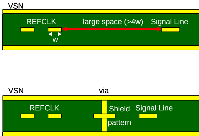
FIGURE 11. SEPARATION OF REFCLK AND OTHER SIGNALS
