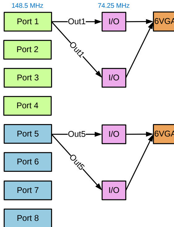
FIGURE 42. PROGRAMMING EXAMPLE 3 : 6VGA, FMI
