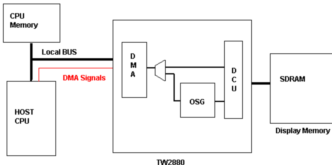
FIGURE 62. DMA OPERATION DIAGRAM
