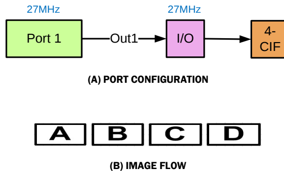
FIGURE 29. PORT SETTING EXAMPLE 5 : 4-CIF
