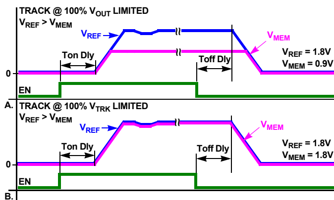
FIGURE 18. COINCIDENT TRACKING
