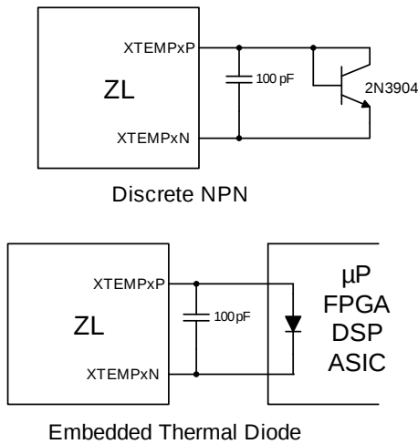
FIGURE 7. EXTERNAL TEMPERATURE MONITORING
