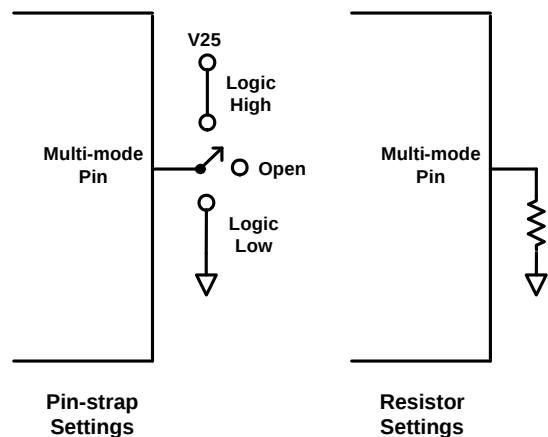
FIGURE 1. PIN-STRAP AND RESISTOR SETTING
