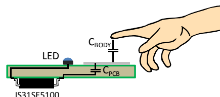
Figure 2: Capacitance Detection
