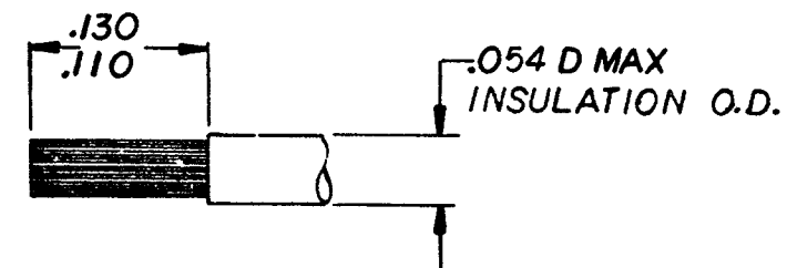
WIRE STRIP DIMENSION
