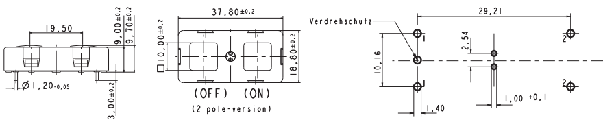
PCB footprint
