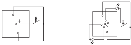
Tactile switch, non-illuminated
