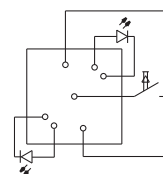
Tactile switch, spot-illuminated
