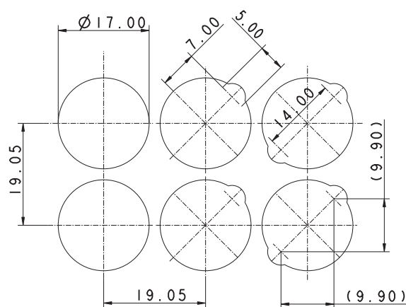
RF 15 N with plunger \varnothing 15 mm, illuminated
