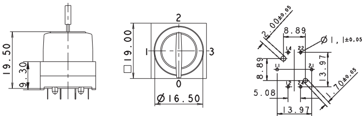
PCB hole pattern, component side
