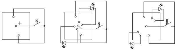
Tactile switch, non-illuminated Tactile switch, fully-illuminated Tactile switch, spot-illuminated
