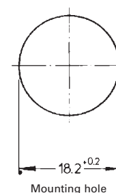
Mounting hole
