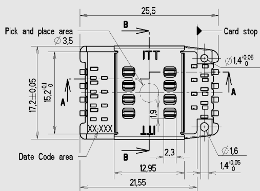
Fixed cover CCM03-3505 (6 contacts not shown) / CCM03-3504 (8 contacts)
