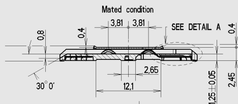
Fixed cover CCM03-3505 (6 contacts not shown) / CCM03-3504 (8 contacts)
