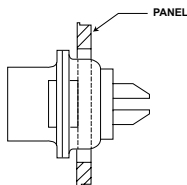
Front mounting of reverse mount shell (Y-Code)
