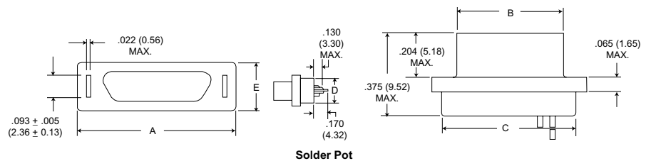
MD Glass-filled Diallyl Phthalate Plastic Insulator
