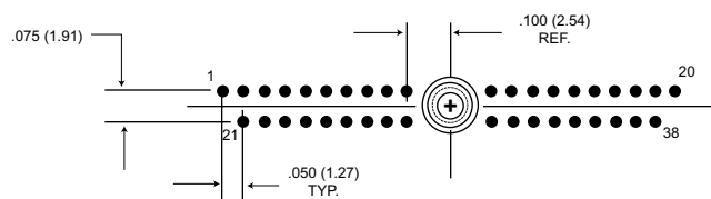
38 Contacts
