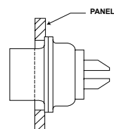
Rear mounting of standard shell
