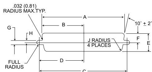
Optional Cutout (For Rear Mounting)
