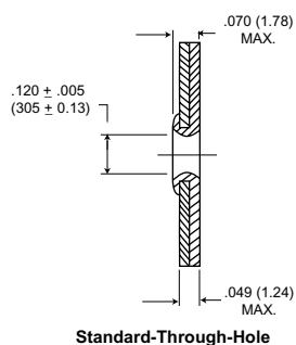
Standard-Through-Hole
