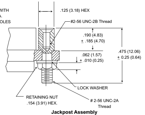
Jackpost Assembly
