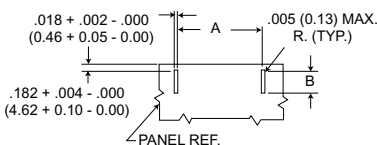
Figure 4 Edgeboard Mounting
