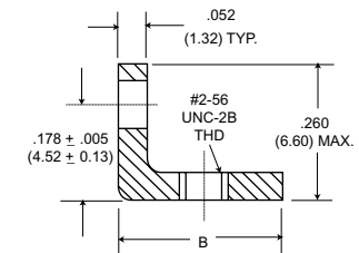
Jackpost - (P)
