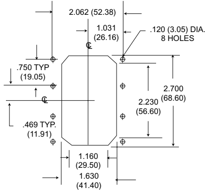
- 33 REAR MOUNT
