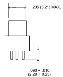
Plug
