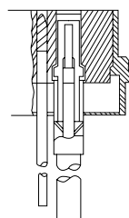
Plug
