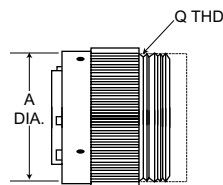
SOLDER KPT06/MS3116
