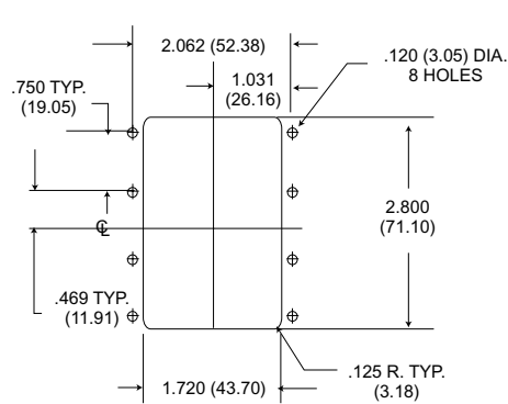
- 33 FRONT MOUNT
