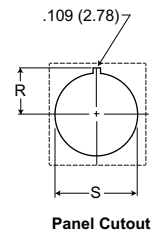
Panel Cutout
