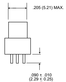
Plug
