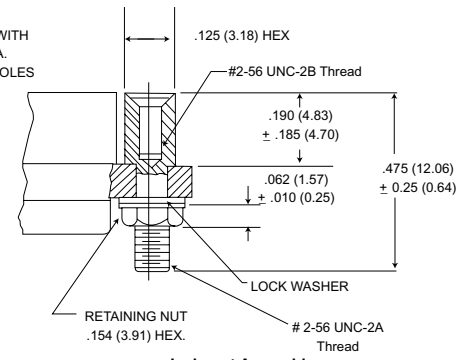
Jackpost Assembly
