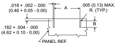
Edgeboard Mounting
