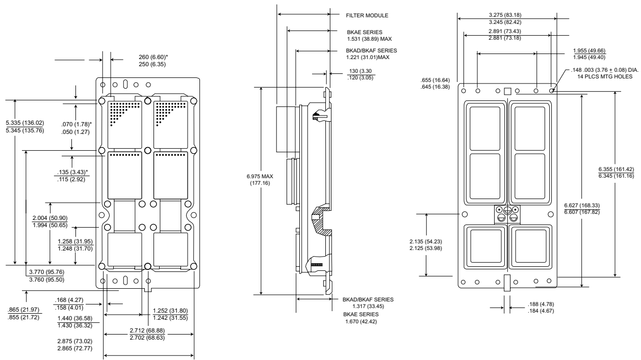
Retainer Plate
