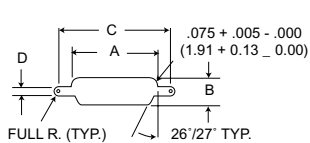
Rear Mounting
