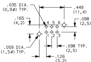
PC MOUNTING
