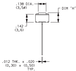
PTS645SL43TR SPST
