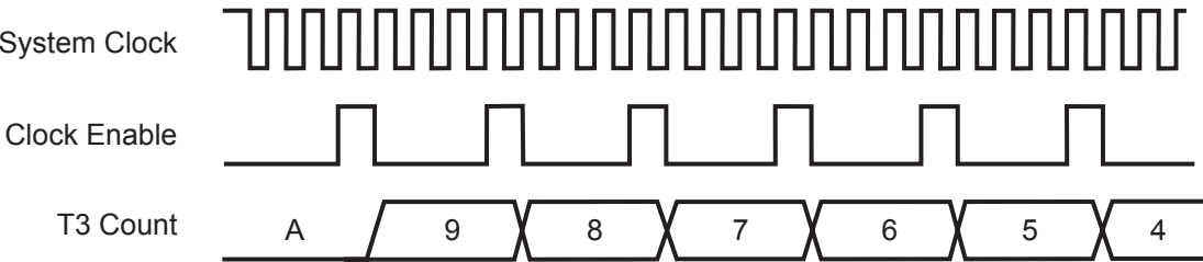
Figure 32. Multi-PWM Operation—Expanded View of Timing
