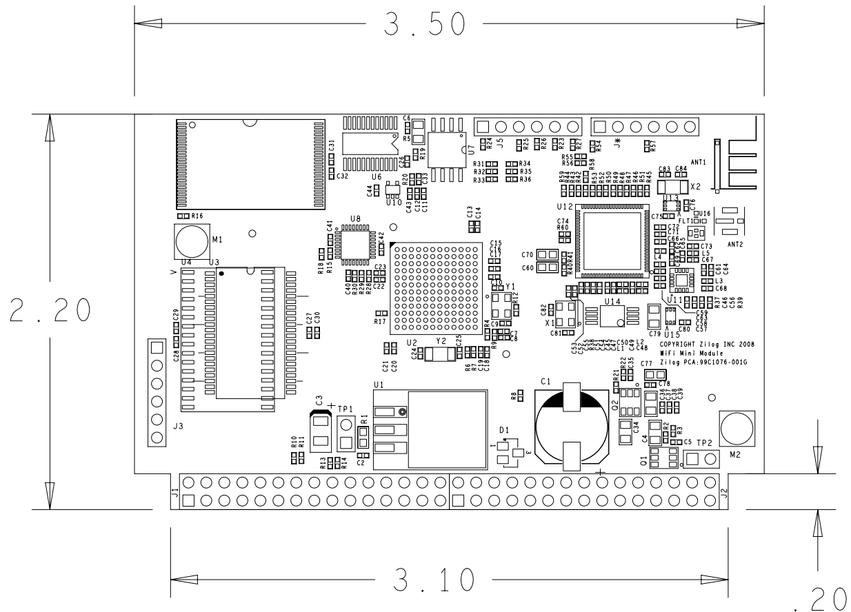
Figure 5. Physical Dimensions of the eZ80AcclaimPlus!™ Wireless Zdots® SBC
