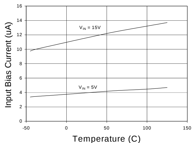
V_{SUPPLY} = 15V
