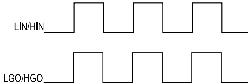
Figure 4. INPUT/OUTPUT Timing Diagram
