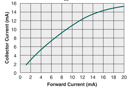
Typical Collector Current vs. Forward Current ( V_{CE}=0.8V )
