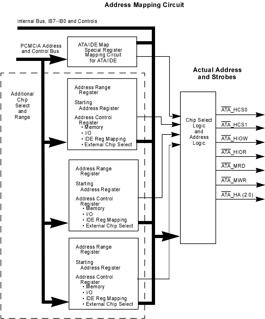
Figure 1. Z86017 Functional Block Diagram
