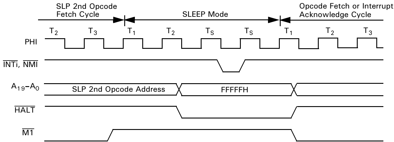
Figure 14. SLEEP Timing
