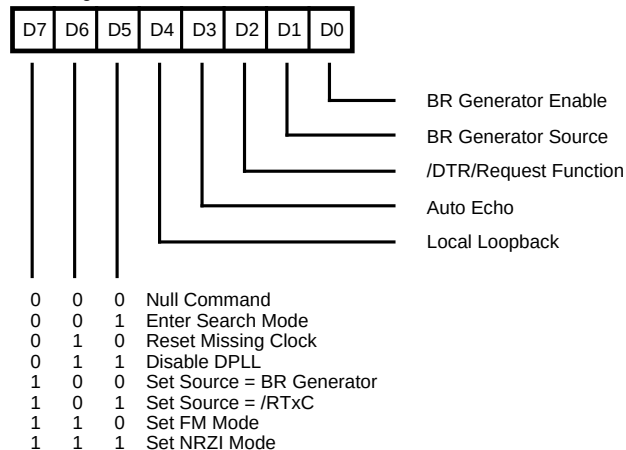
Write Register 14
