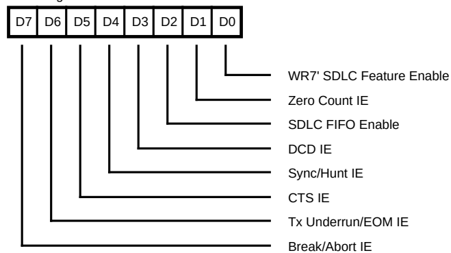
Write Register 15
