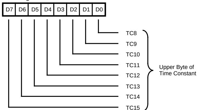
Write Register 13
