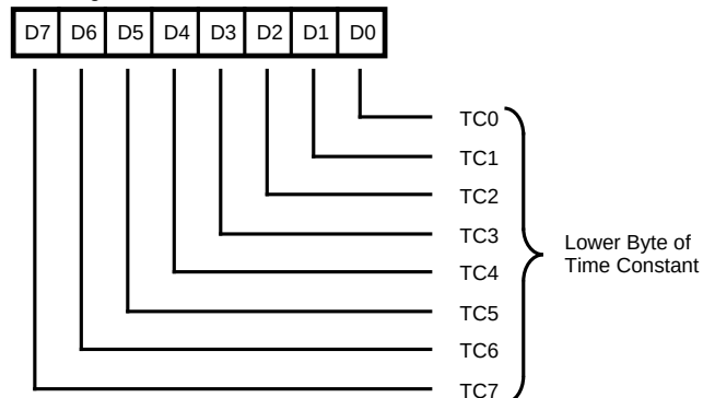
Write Register 12
