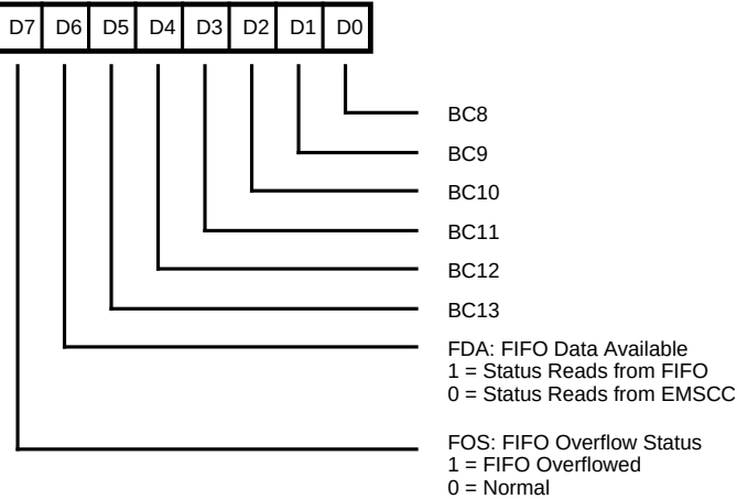
Read Register 7*
