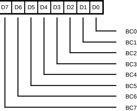
Read Register 6*
