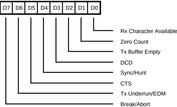
Read Register 0
