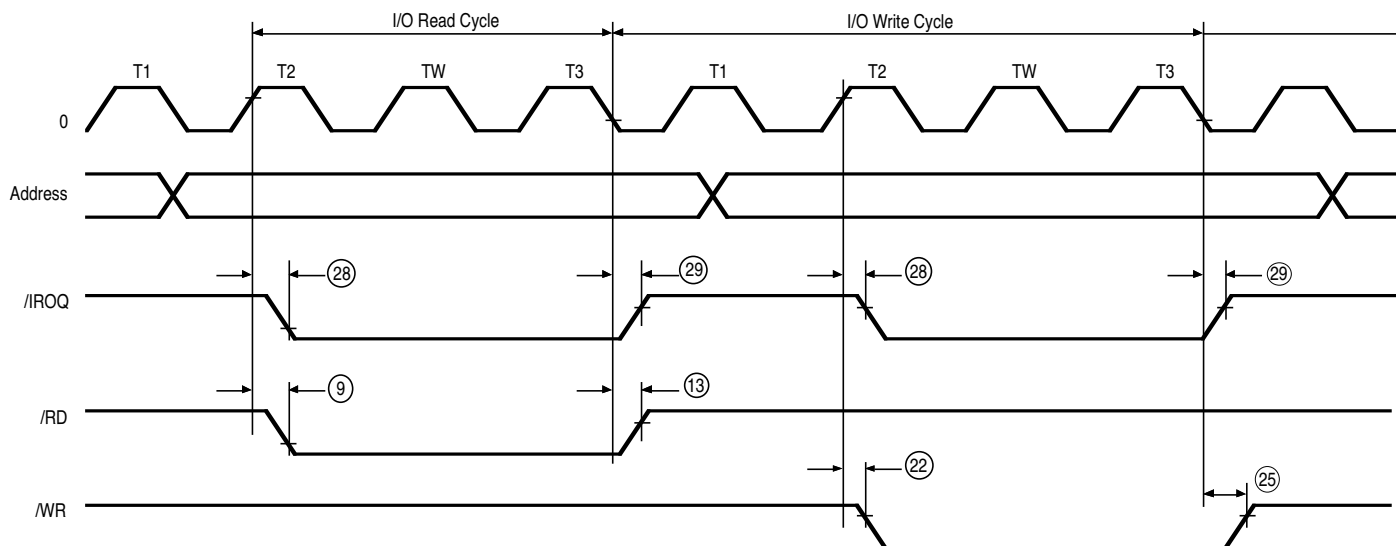
Figure 92. CPU Timing
