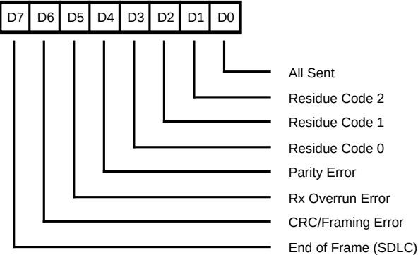
Read Register 1
