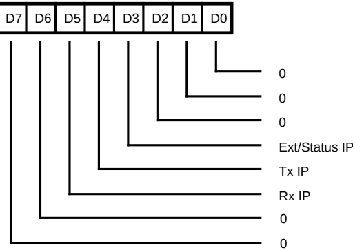
Read Register 3
