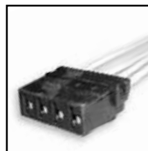
2899-1F Ford Fan Switch Repair Harness 12085487
