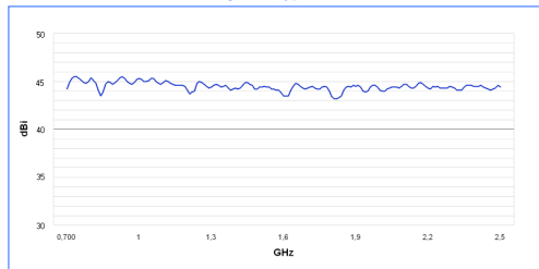
Gain diagram HyperLOG 7025X
