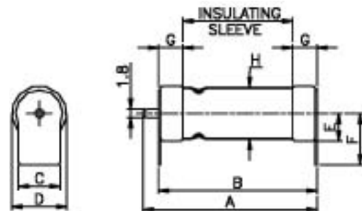
Fig. 6 Case Sizes - Outline and Dimensions
