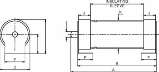
SMTH Fig. 2. Case Sizes - Outline and Dimensions
