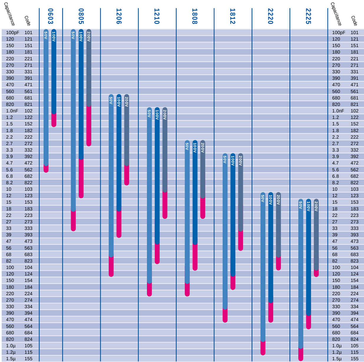
2C1 (BZ) capacitor range
