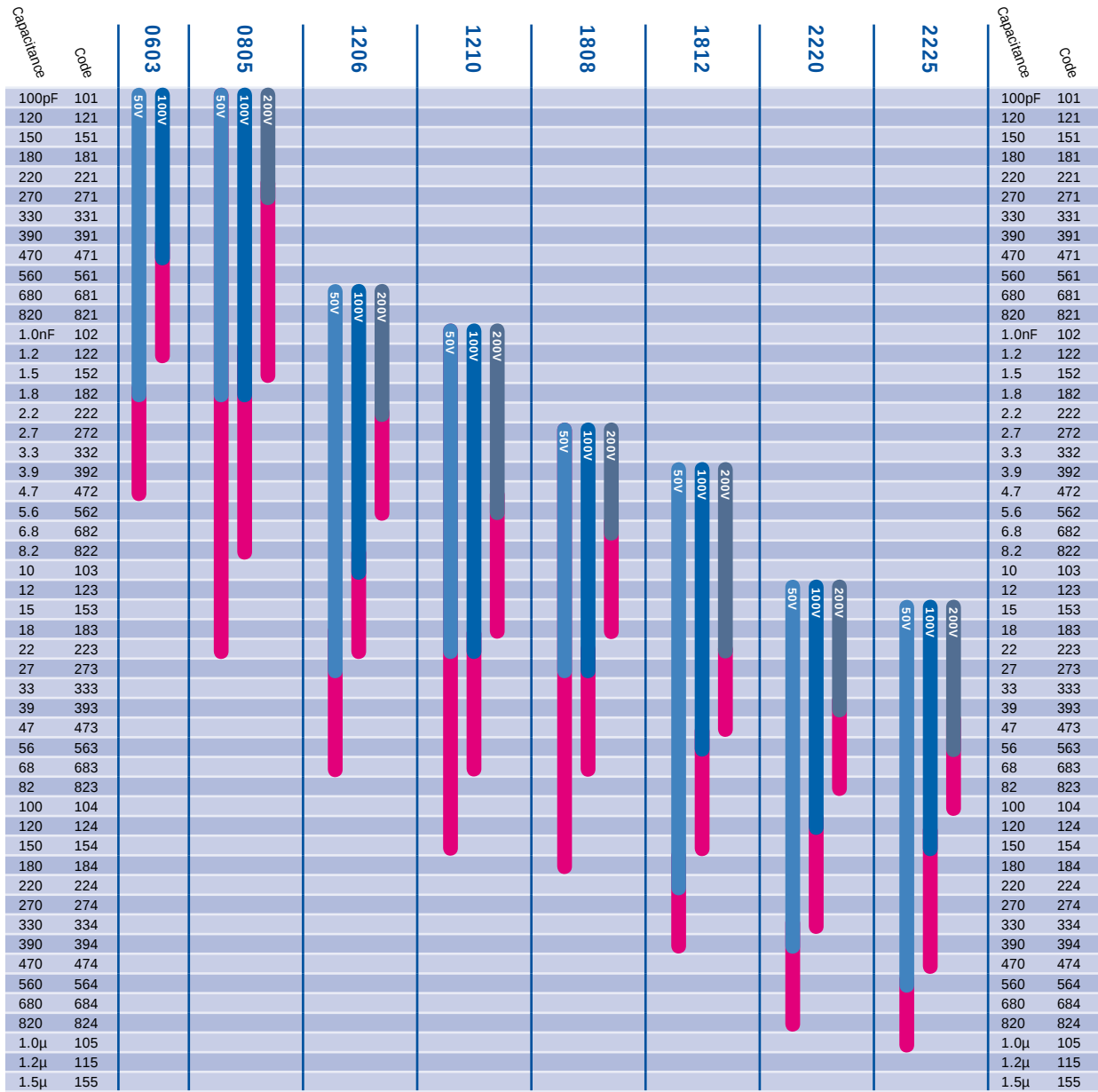
2X1 (BX) capacitor range
