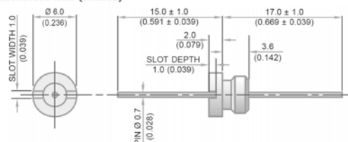
Dimensions mm (inches)
