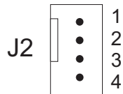
Figure 11: PWM Fan Connector J2
