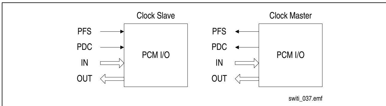
Figure 10 PCM Interface Configurations
