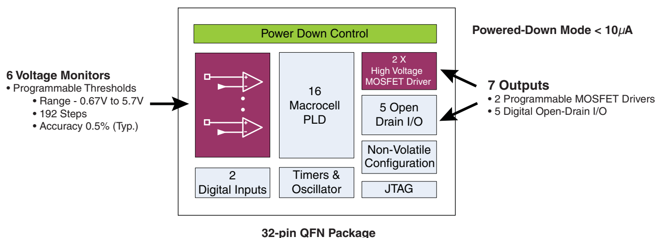
Figure 1-6. Block Diagram of an ispPAC-POWR607 Device
