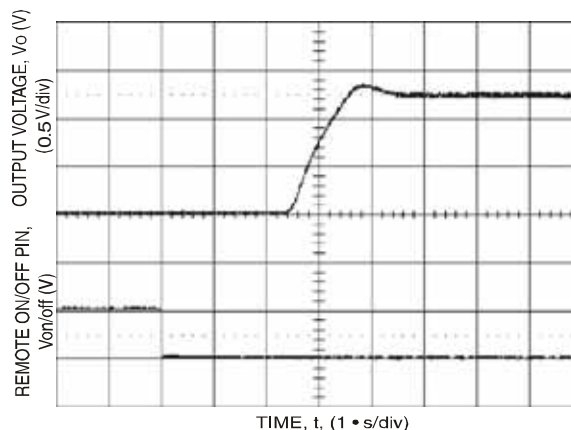
Figure 6. Start-up from Remote On/Off ( I_O = I_{O, \text{max}} ).
