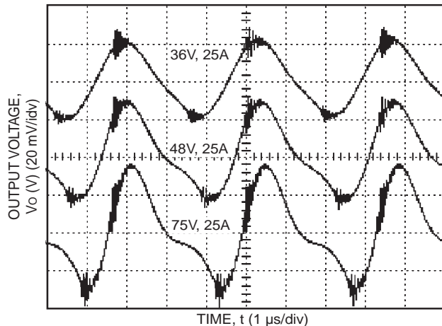
Figure 9. Output Ripple Voltage ( I_O = I_{O, \text{max}} ).
