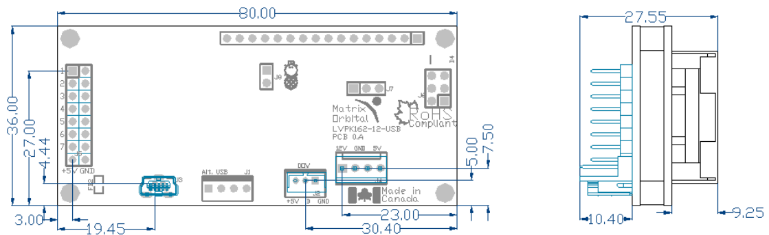
Figure 21: LK162-12-USB Dimensional Drawing
