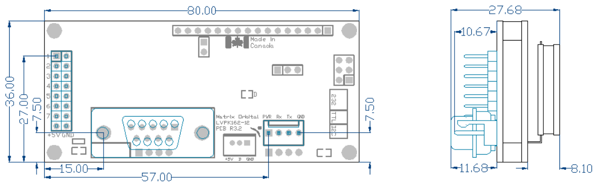
Figure 23: VK162-12 Dimensional Drawing
