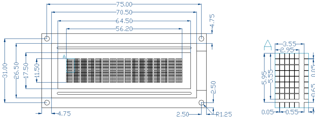
Figure 19: LK162-12 Screen Drawing
