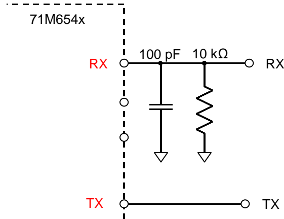
Figure 40: Connections for UART0
