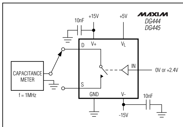
Figure 6. Source/Drain Off-Capacitance
