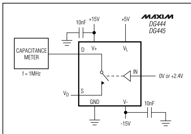
Figure 7. Source/Drain On-Capacitance
