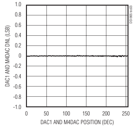
DAC1 AND M4DAC DNL
