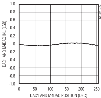
DAC1 AND M4DAC INL
