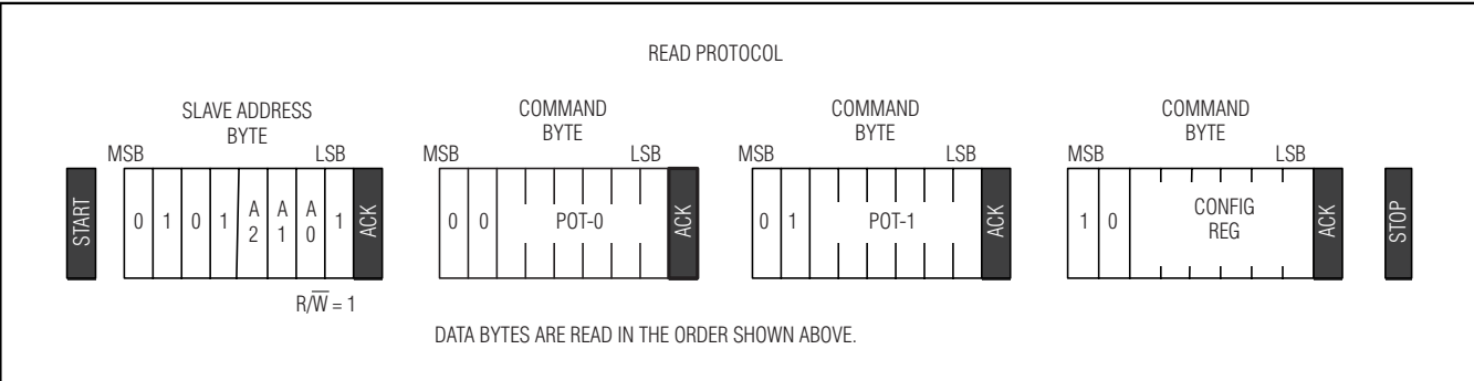
Figure 1. Read Protocol
