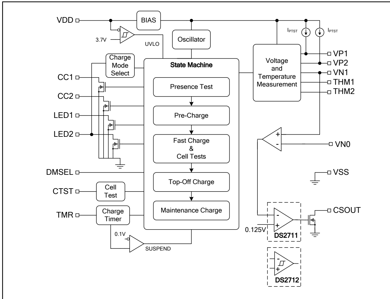
Figure 1. Block Diagram
