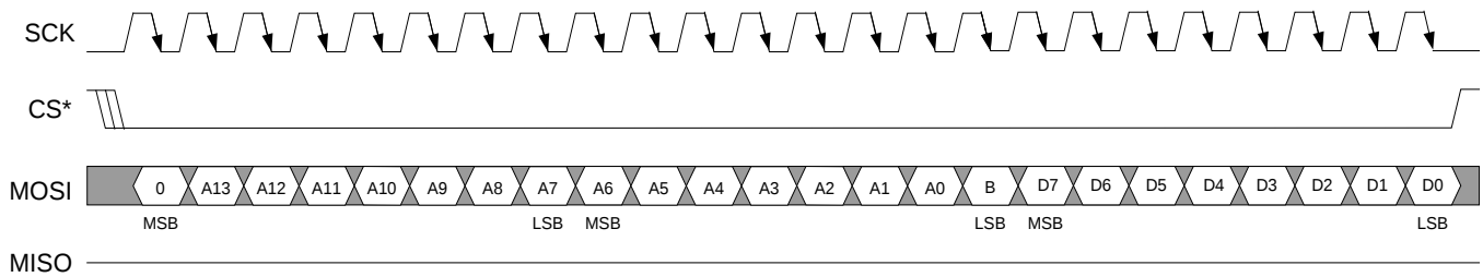
Figure 8-26. SPI Serial Port Access For Write Mode, SPI_CPOL = 1, SPI_CPHA = 1
