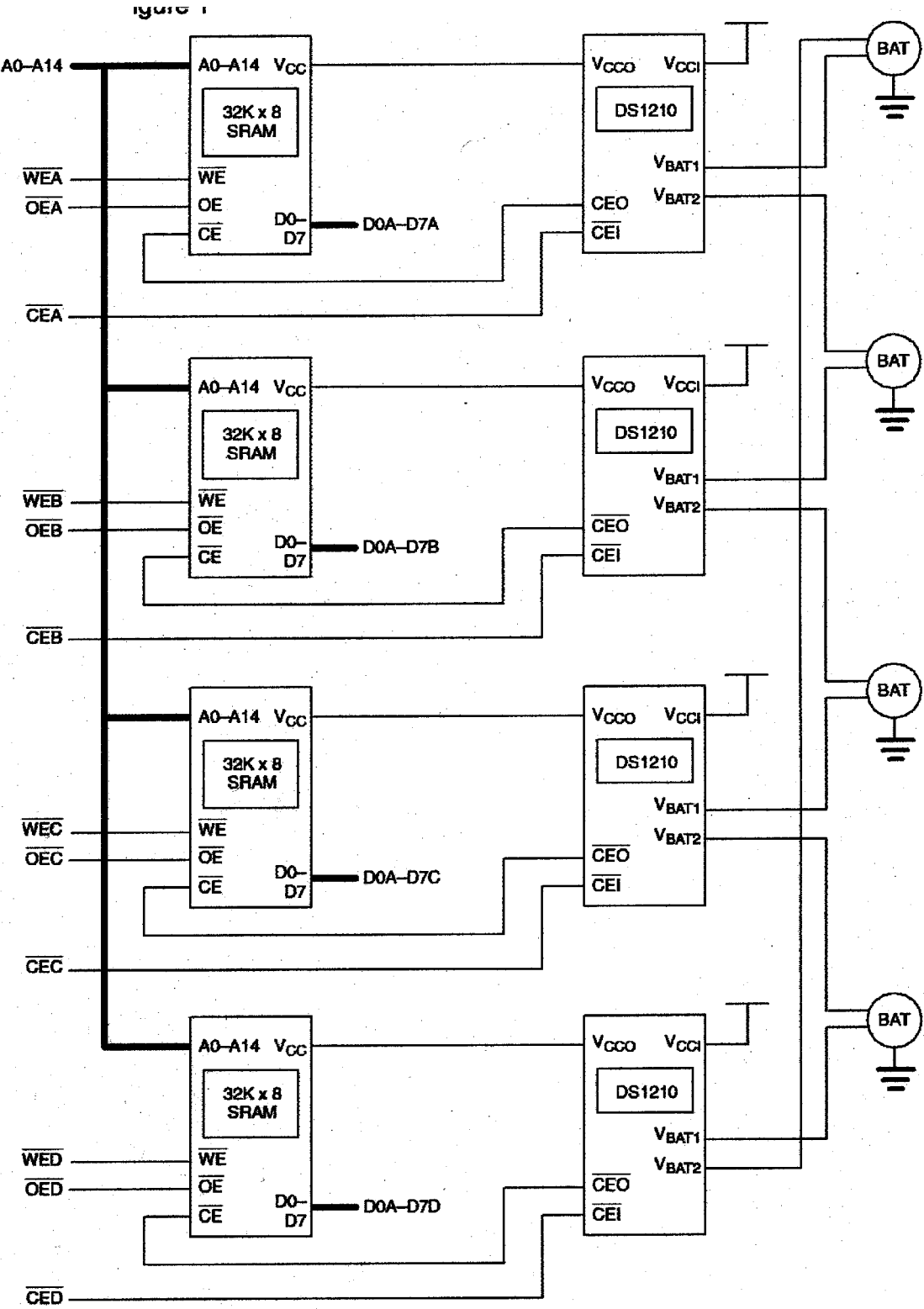
BLOCK DIAGRAM Figure 1
