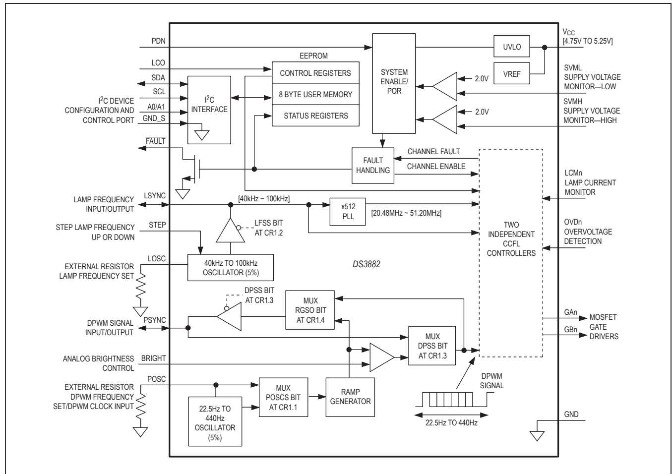
Figure 1. Functional Diagram
