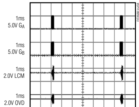
BURST DIMMING AT 150Hz AND 10%
