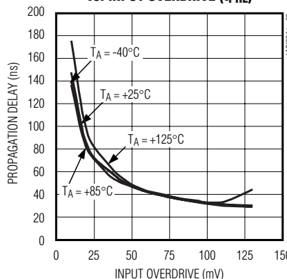
PROPAGATION DELAY vs. INPUT OVERDRIVE ( t_{PHL} )
