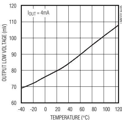
OUTPUT LOW VOLTAGE vs. TEMPERATURE
