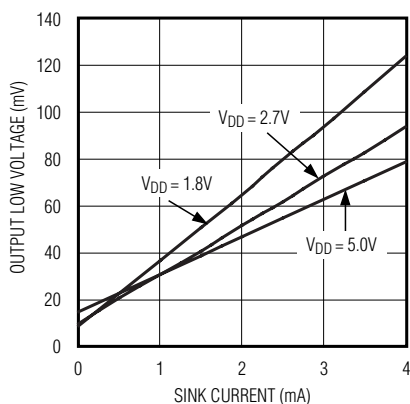
OUTPUT LOW VOLTAGE vs. SINK CURRENT
