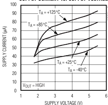
LMX331 SUPPLY CURRENT vs. SUPPLY VOLTAGE
