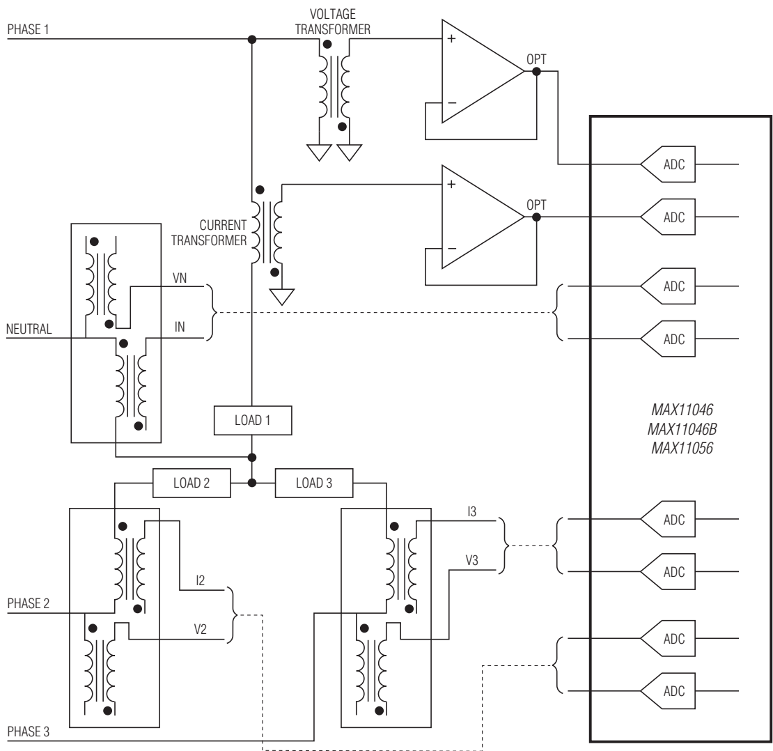
Figure 10. Power-Grid Protection
