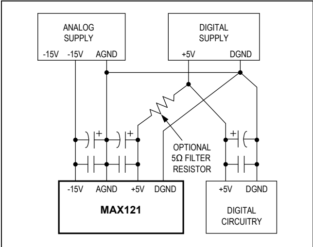
Figure 26. Power-Supply Grounding
