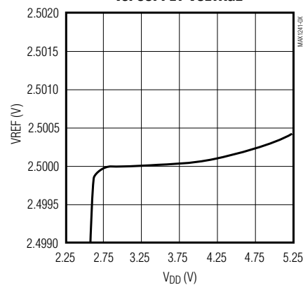
MAX1240 INTERNAL REFERENCE VOLTAGE vs. SUPPLY VOLTAGE
