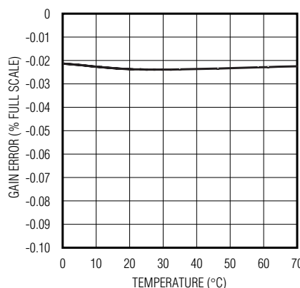
MAX1493/MAX1495 GAIN ERROR vs. TEMPERATURE
