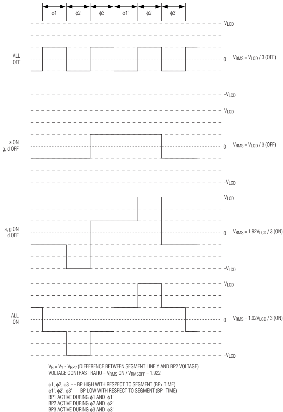
Figure 11. Voltage Waveforms on the g Segment
