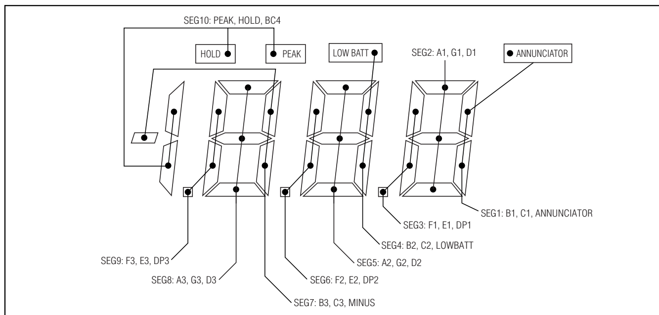
Figure 7. Segment Connection for the MAX1491 (3.5 Digits)
