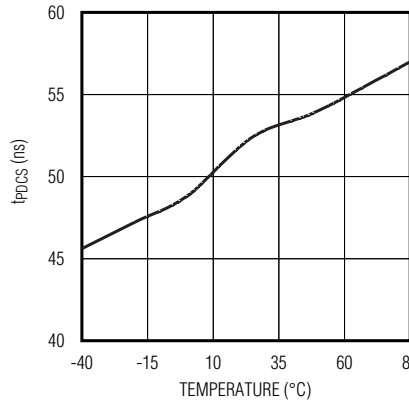
PROPAGATION DELAY FROM CURRENT-LIMIT COMPARATOR INPUT TO NDRV vs. TEMPERATURE
