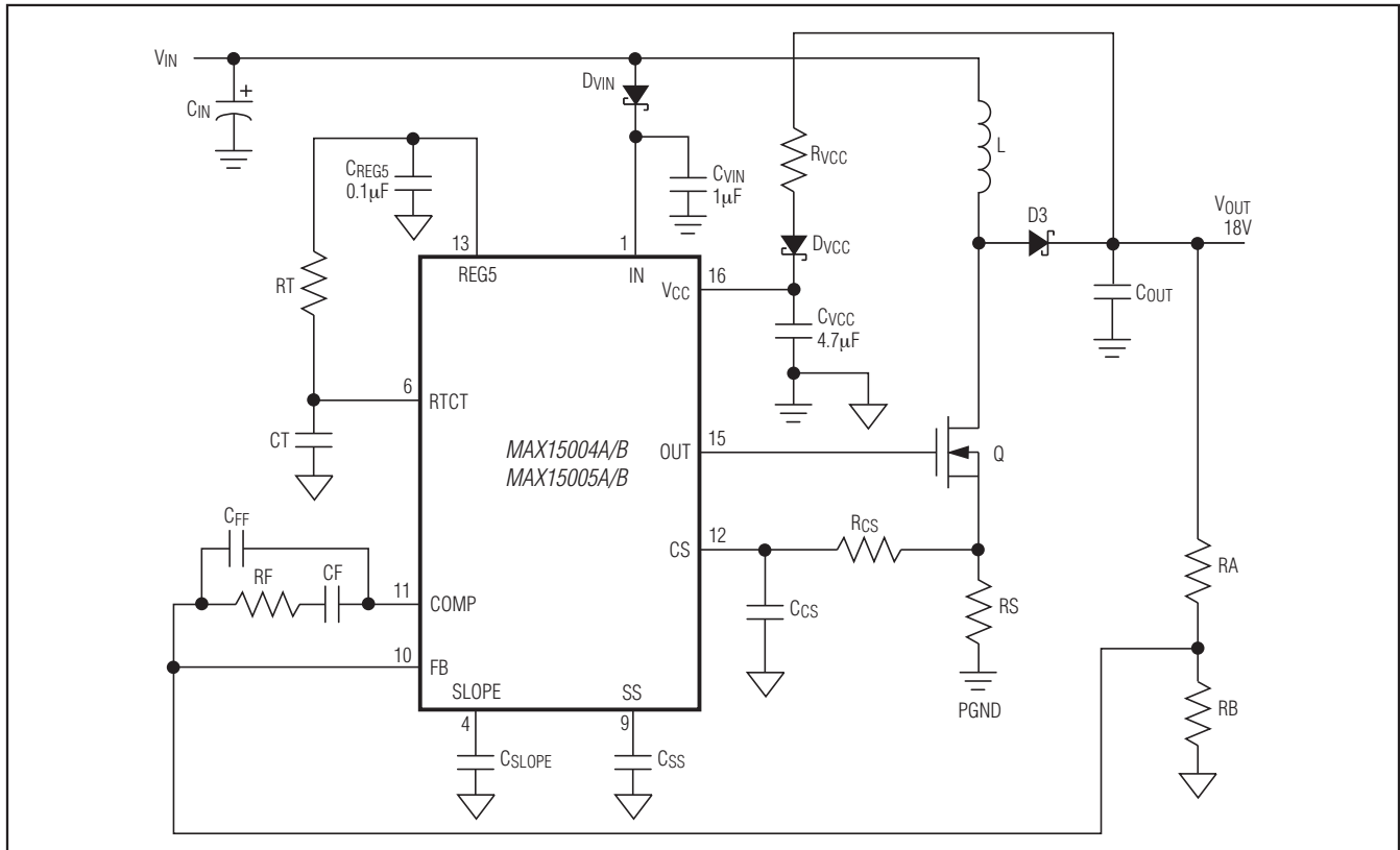
Figure 5. Application Schematic
